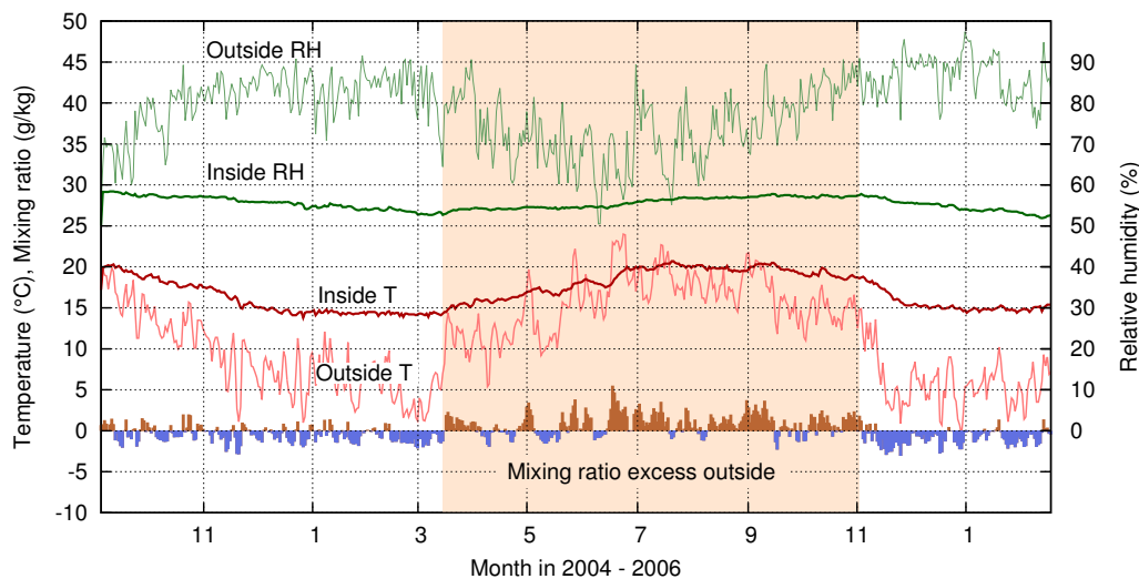
Figure 5: The RH in the Suffolk Record Office, UK. In this building there is no dehumidification; the moderate annual RH is attained by winter heating to a minimum 15 °C. The RH continues steady over the summer months even though the mixing ratio shows an almost continuously higher concentration of water vapour outside, which would raise the interior RH as it leaked in. The humidity buffering by the abundant paper prevents significant change of RH.
