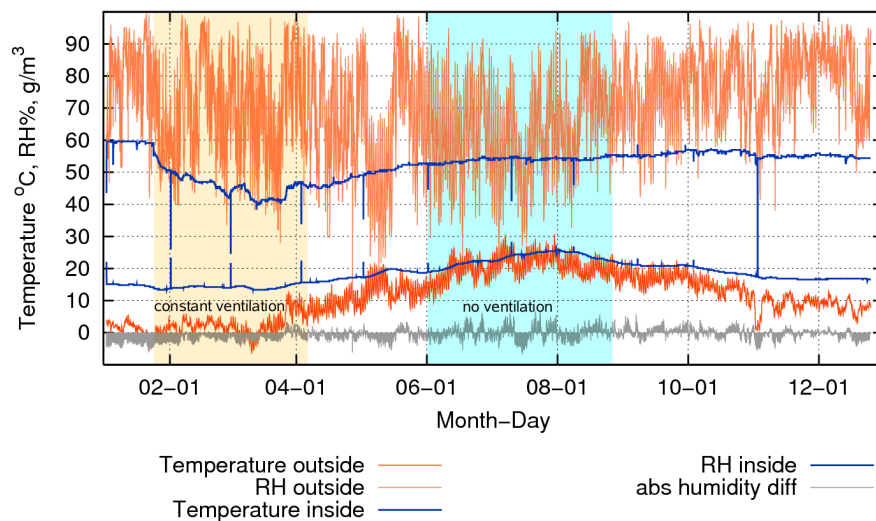
Figure 7: The climate inside and outside the Arnemagnaeen archive during tests in 2006 of its resistance to malfunction of the air pumping system. The decrease in inside RH during February and March was caused by deliberately ventilating the room continuously, at 2 air changes per hour, to stress the humidity buffering. During July and August the room was completely unventilated, to test the resistance to the high RH expected in summer. The grey trace at the bottom shows the difference between outside and inside water vapour concentration. Shading above the zero line indicates a higher water vapour concentration outside. The sharp blips on the curves mark short periods when the data logger was withdrawn to the conservator's office for the data to be extracted. These brief retreats reveal the temperature and RH which surrounds six of the eight sides of the archive.
