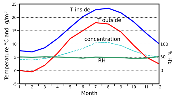
Figure 11: The curves in this graph are derived from the monthly average temperature and RH in Copenhagen over the last 30 years. A room has to be heated to lower the RH. The inside temperature is a sine curve, which gives a RH very close to a constant 50%.
