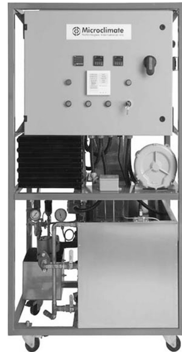
Figure 5. Recent model of a remote positive pressure unit, 2005
