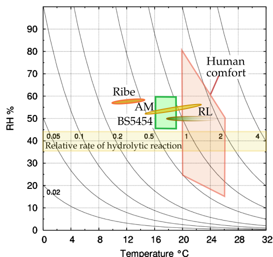
Figure 7: The British Standard for archives, BS 5454:2000, and the climate ranges of the three studied buildings, are superimposed on the Sebera type diagram introduced in Fig. 2. RL: Royal Library, AM: Arnamagnæan archive.
