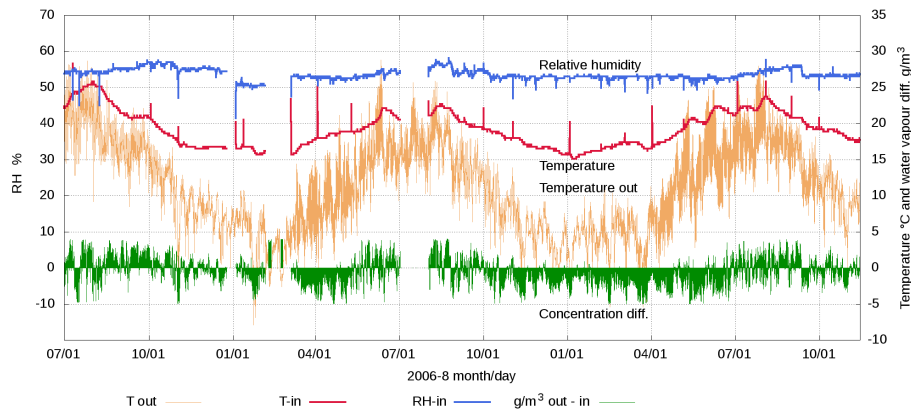
Figure 4: The climate within the Arnamagnæan archive. The lowest trace is the difference between the water vapour concentrations inside and out. When the shaded area is below zero, there is excess water vapour within the archive.
