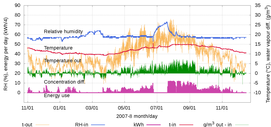
Figure 6: The climate in the Ribe store generally has a constant RH with an annual temperature cycle between 10°C and 15°C. However, when the equipment fails, particularly in summer, the RH rises quite quickly, indicating inadequate humidity buffering for fail-safe operation.
