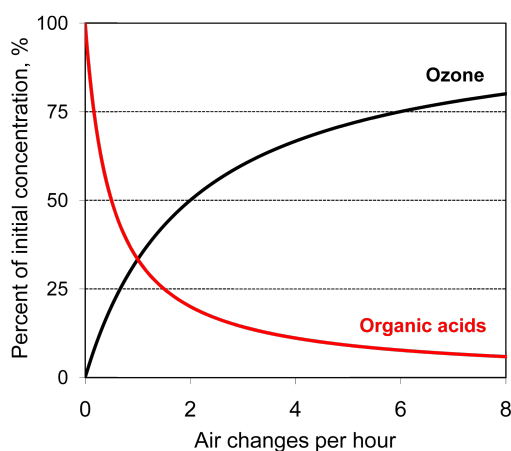
Figure 9: The indoor pollution concentration depends on the air exchange rate. For chemicals generated indoors, the starting point is the steady-state concentration at near-zero ventilation (100%). For compounds such as acetic acid this may be several hundred ppb. Outdoor pollutants decrease in concentration (from an ambient level of 100%) as they are absorbed by deposition on surfaces on their route into a building and within the room. A low air exchange rate retards ingress from outdoors, but at the same time blocks the escape of internally generated pollutants. The model is based on a room comparable to the Arnamagnæan archive, and assumes steady state conditions for outdoor and indoor generation of pollutants (Ryhl-Svendsen 2006).
